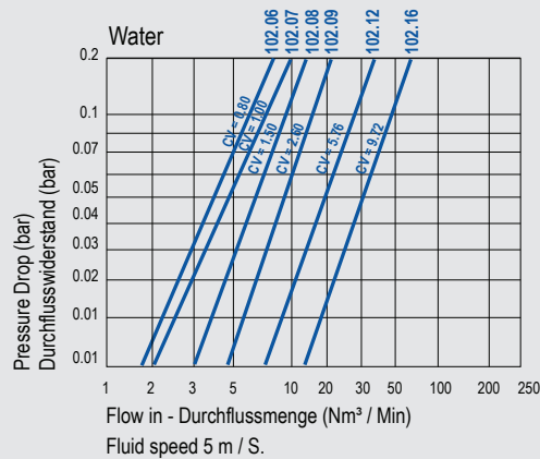
Flow Rate vs Pressure Drop Graph
