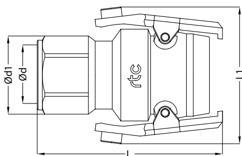
Socket / Kupplung
