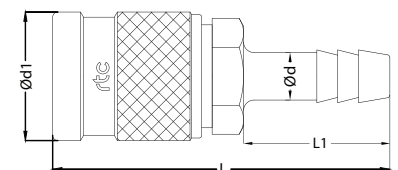
Free-Flow Coupling Kupplung ohne Ventil
