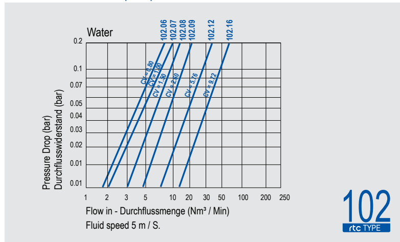
Flow Rate vs Pressure Drop Graph
