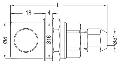
Sockets / Kupplungen
