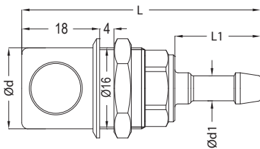
Sockets / Kupplungen
