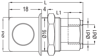
Sockets / Kupplungen
